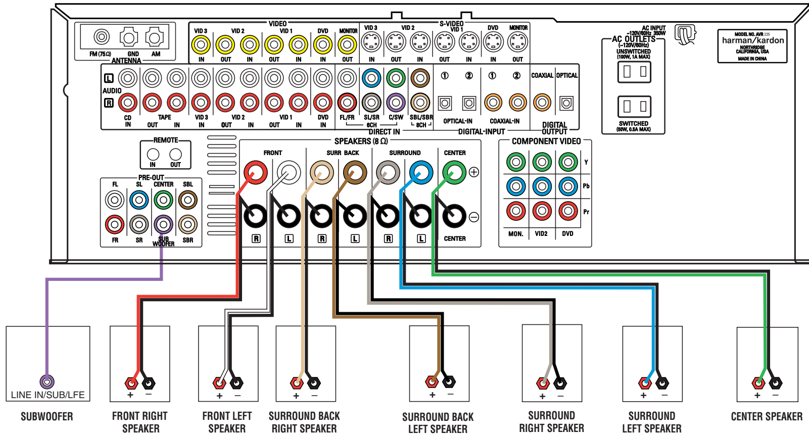
Figure 2 – Speaker Connections
